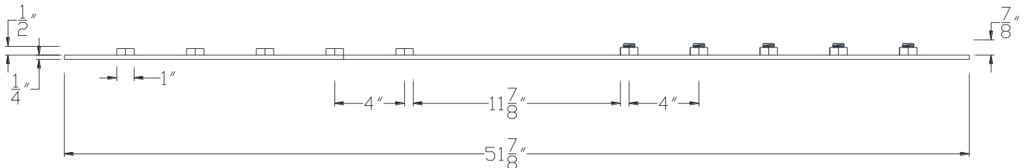
SIDE VIEW
