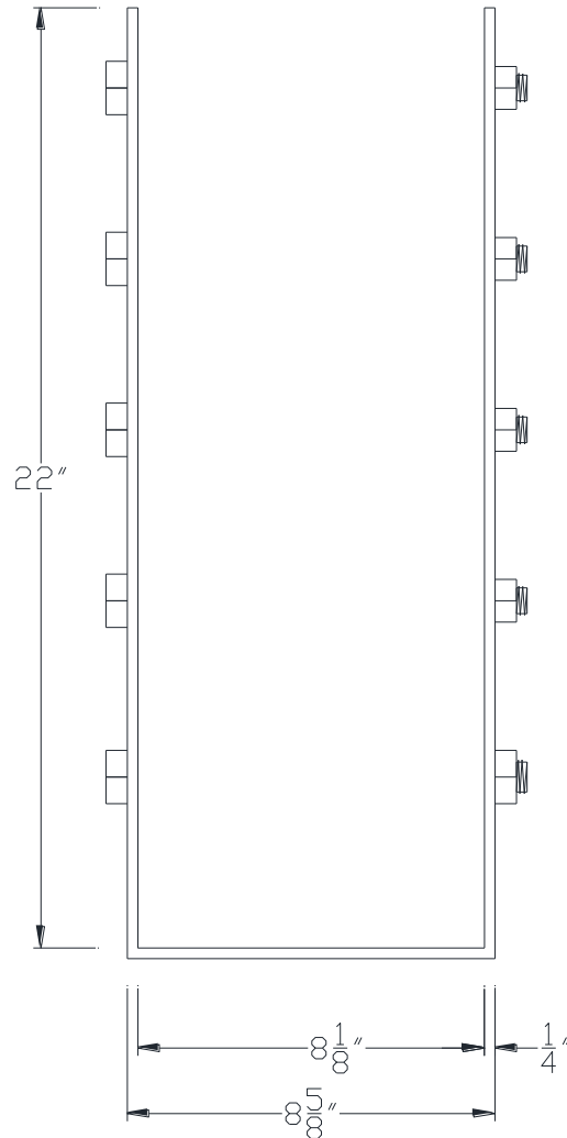
FRONT VIEW
