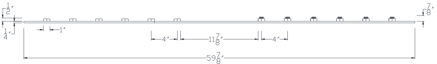
SIDE VIEW
