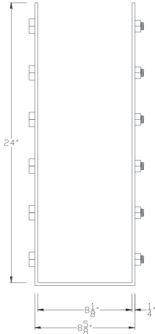
FRONT VIEW
