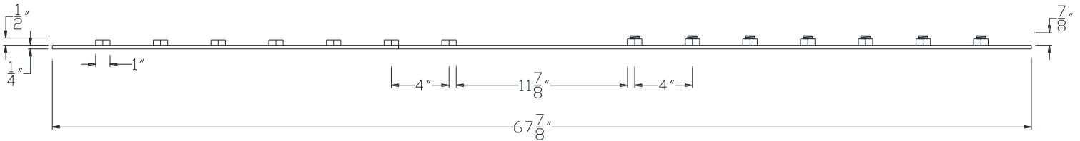
SIDE VIEW
