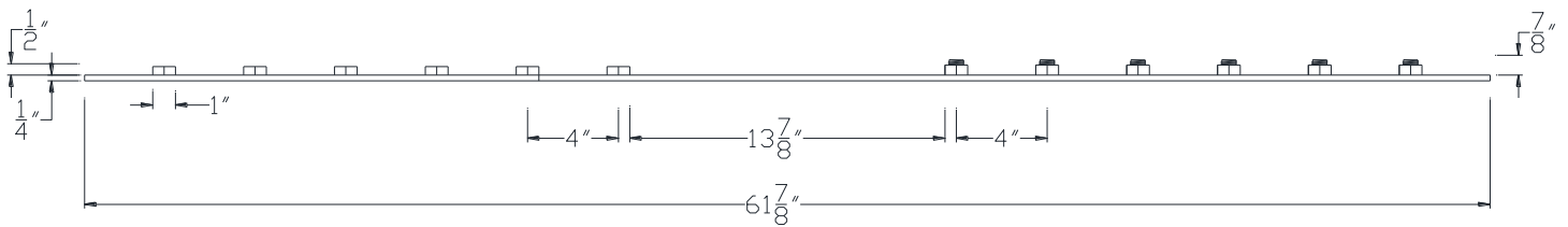
SIDE VIEW
