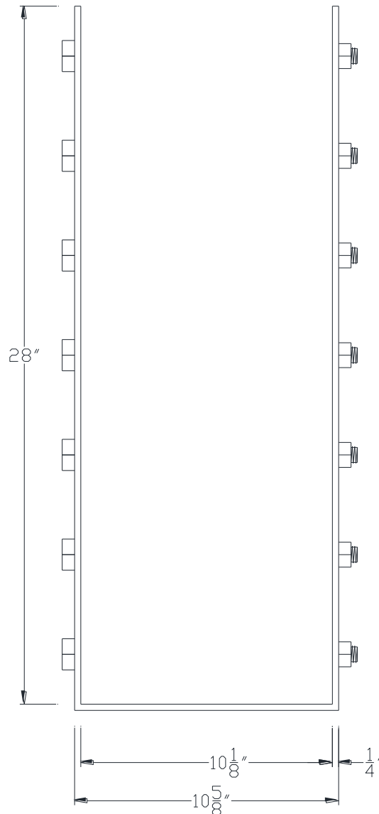
FRONT VIEW
