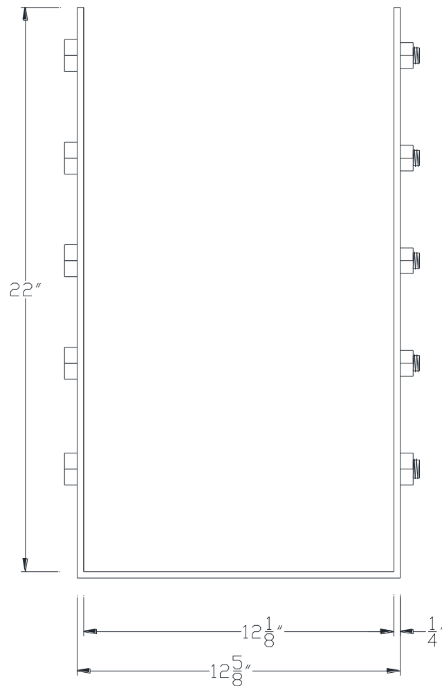
FRONT VIEW
