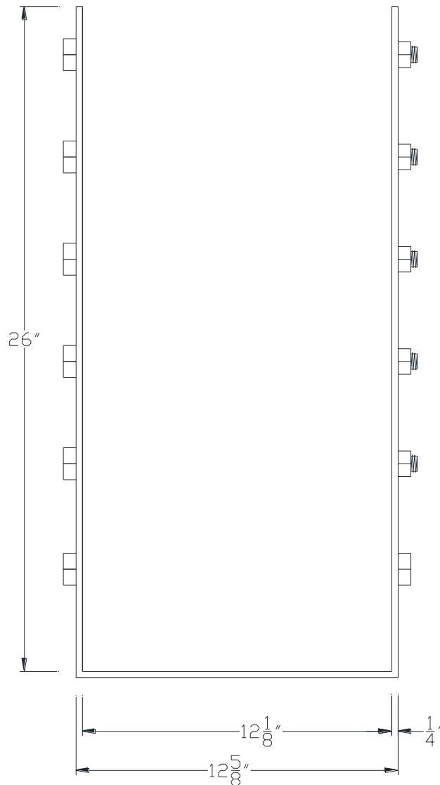
FRONT VIEW
