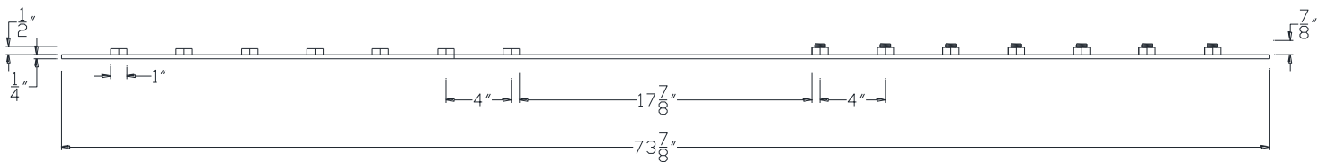
SIDE VIEW
