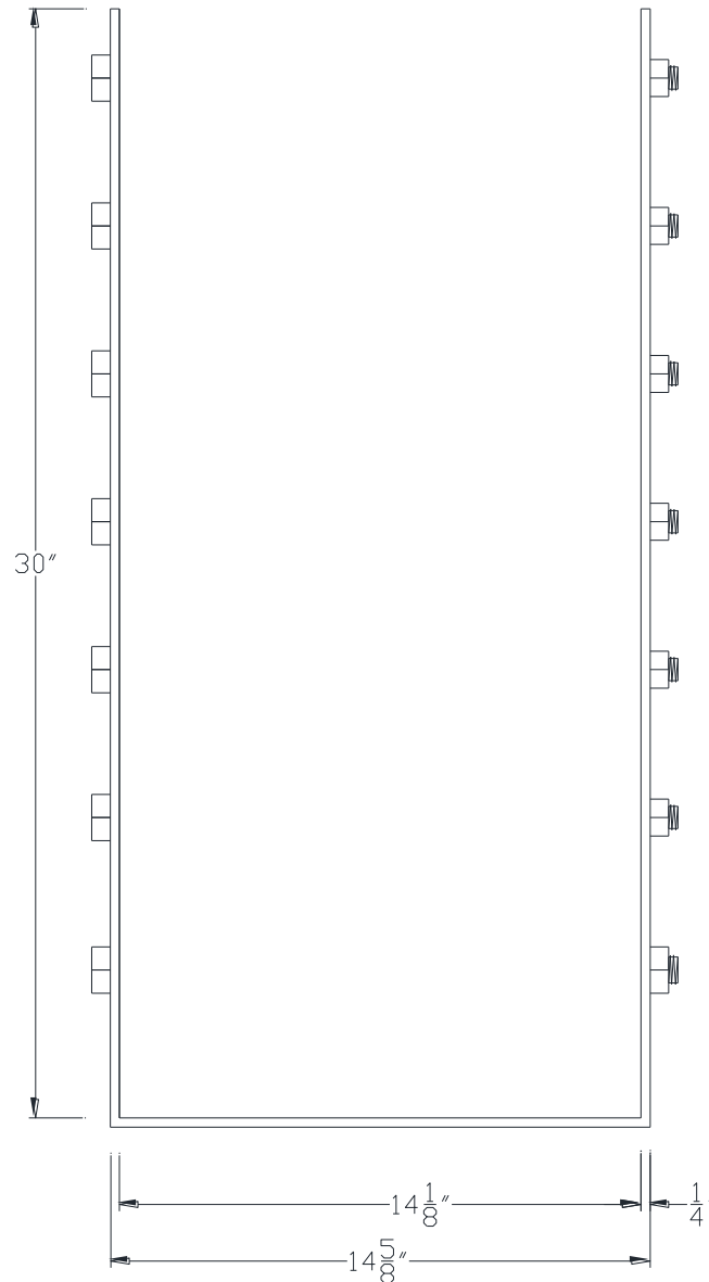
FRONT VIEW
