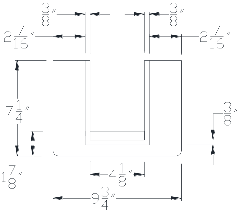
FRONT VIEW
