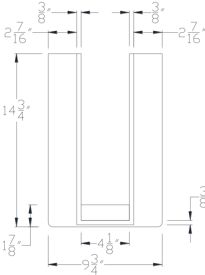
FRONT VIEW
