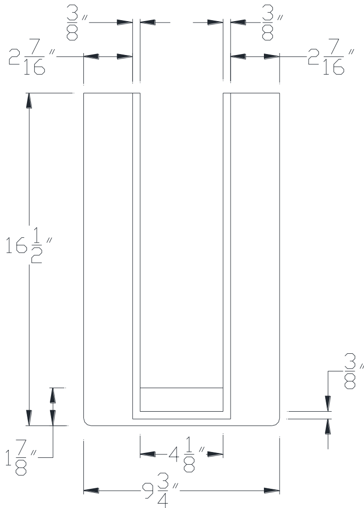
FRONT VIEW
