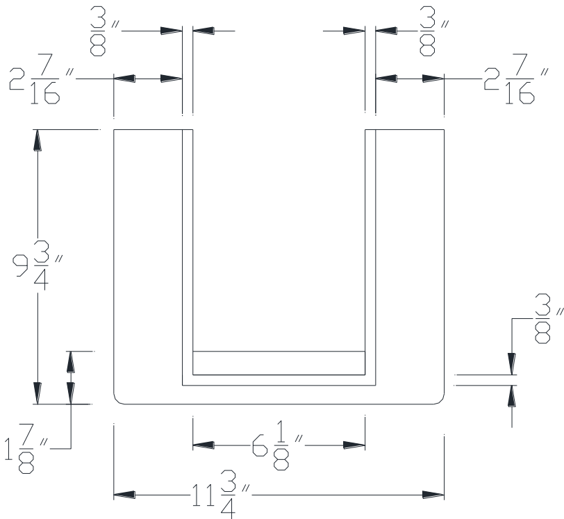
FRONT VIEW
