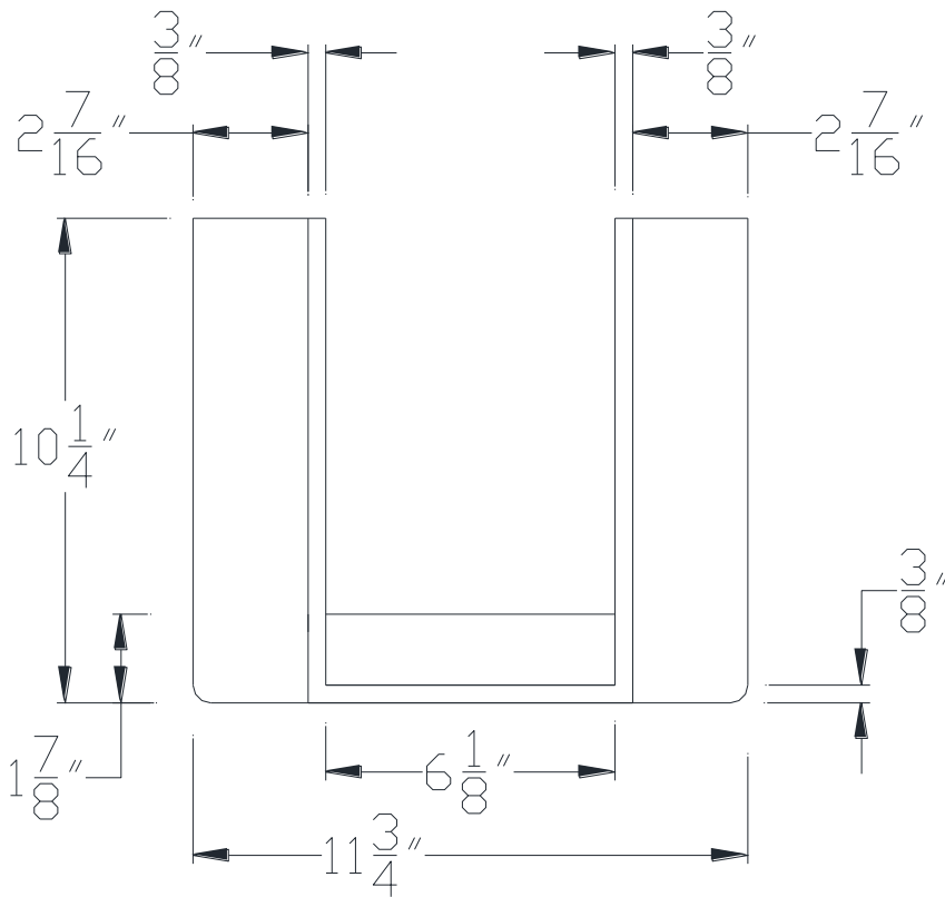
FRONT VIEW
