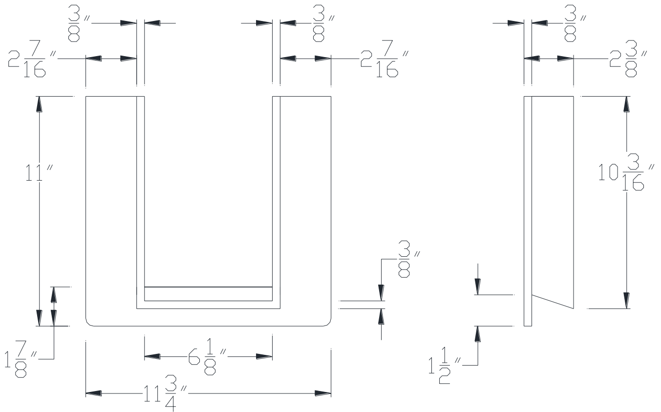
FRONT VIEW
