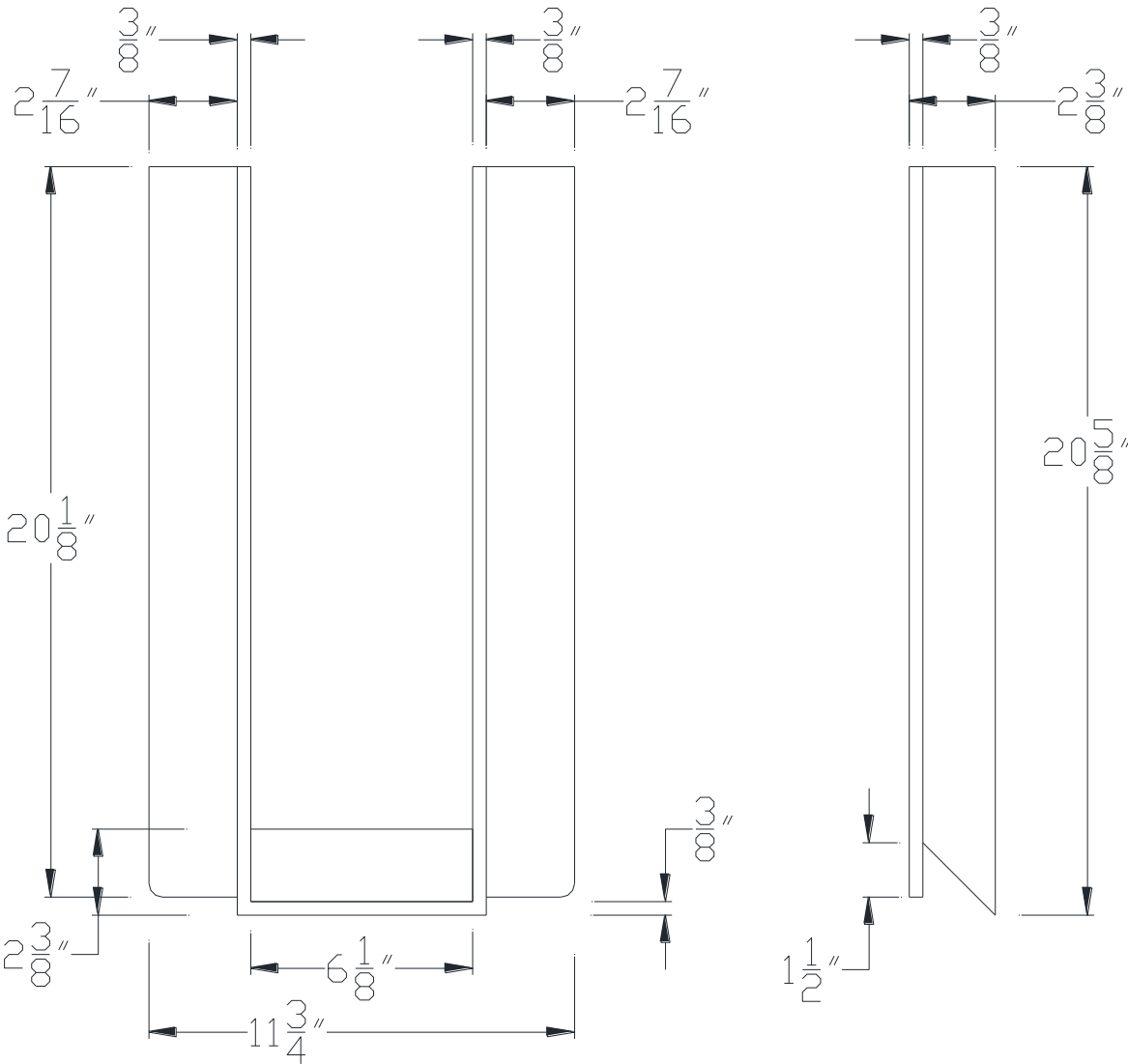
FRONT VIEW
