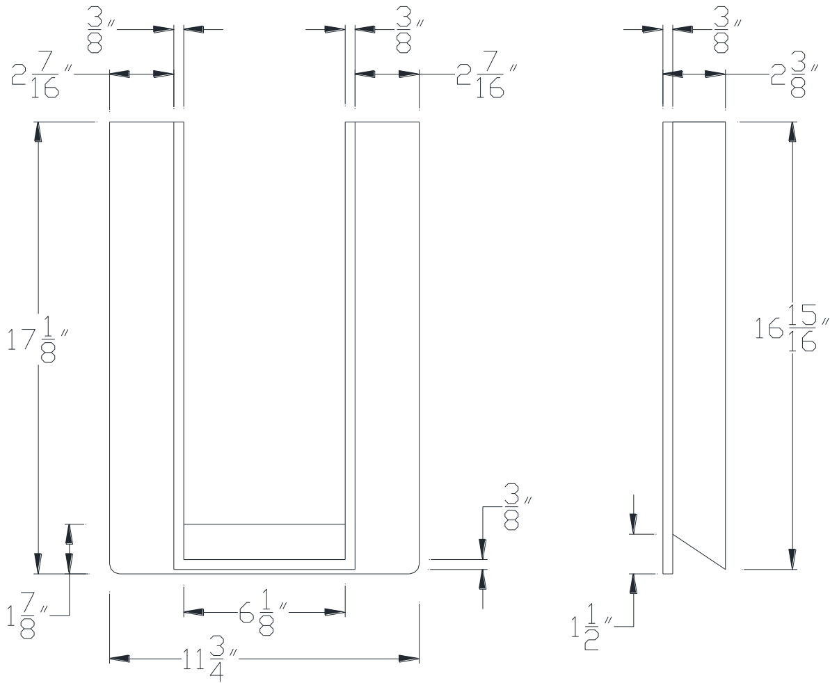
FRONT VIEW
