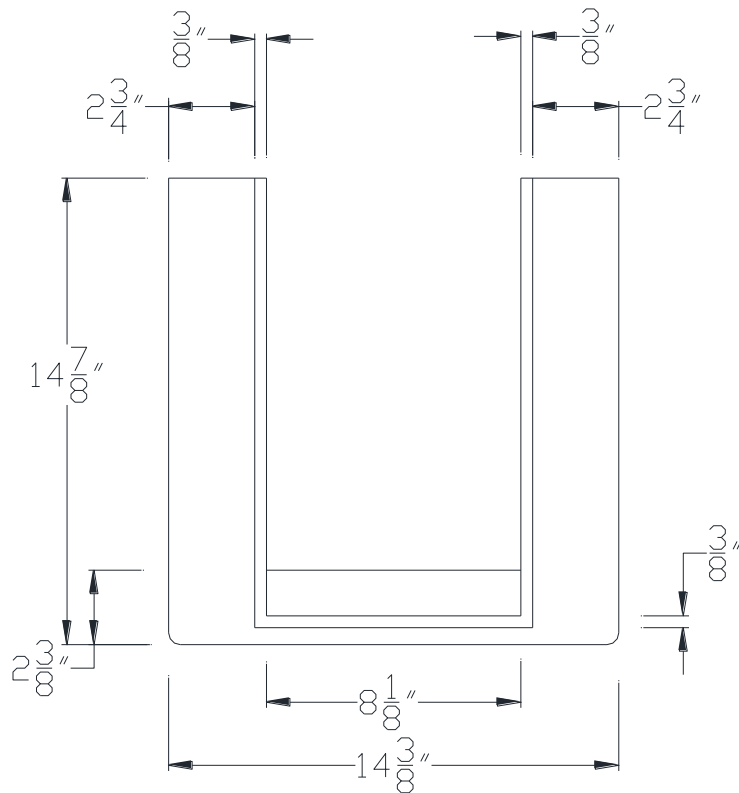
FRONT VIEW
