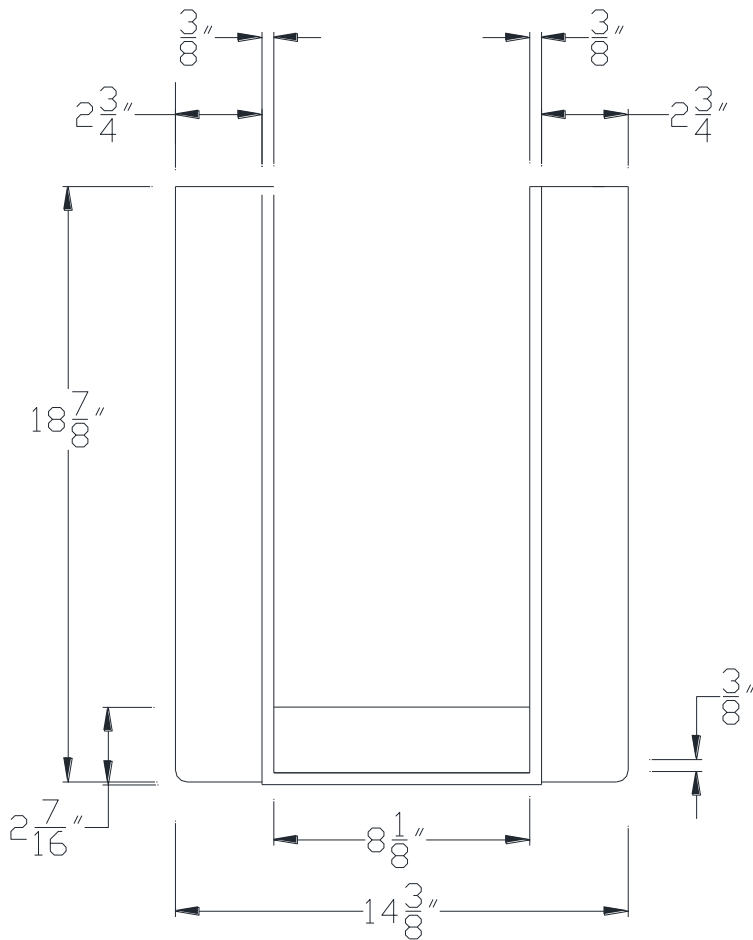
FRONT VIEW
