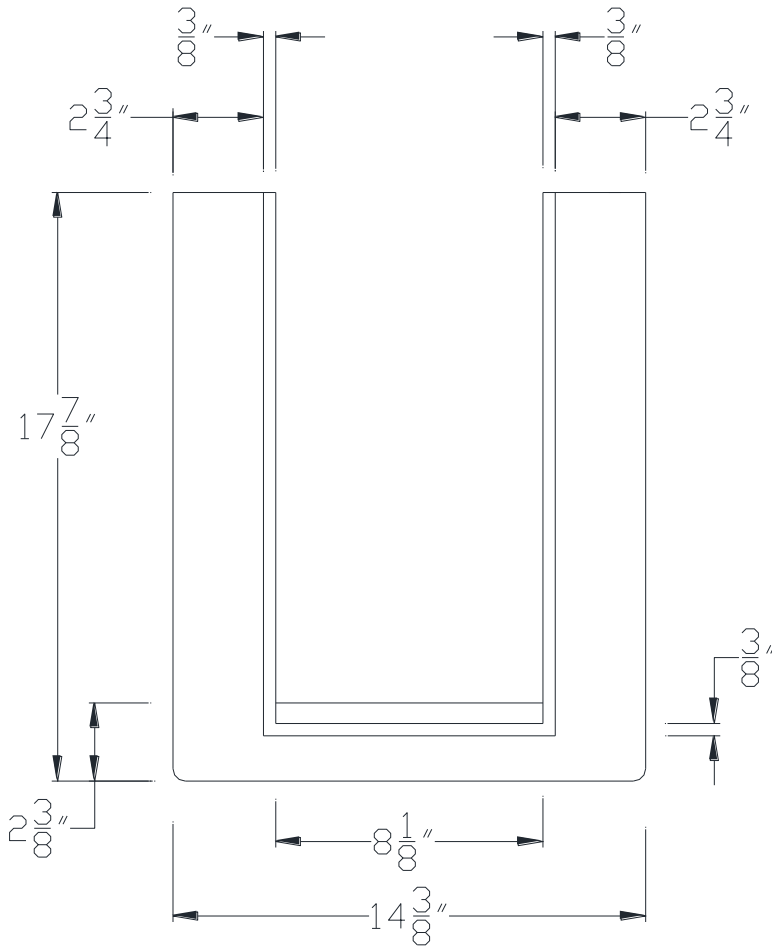
FRONT VIEW
