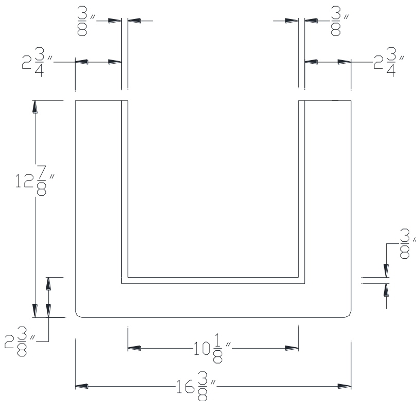
FRONT VIEW
