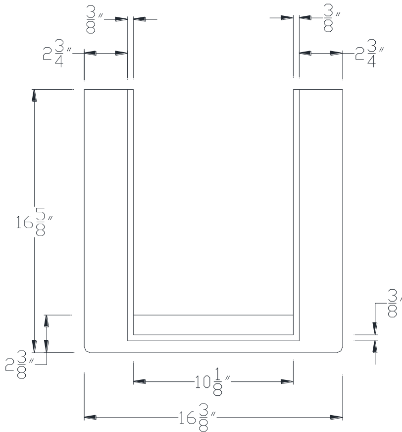
FRONT VIEW
