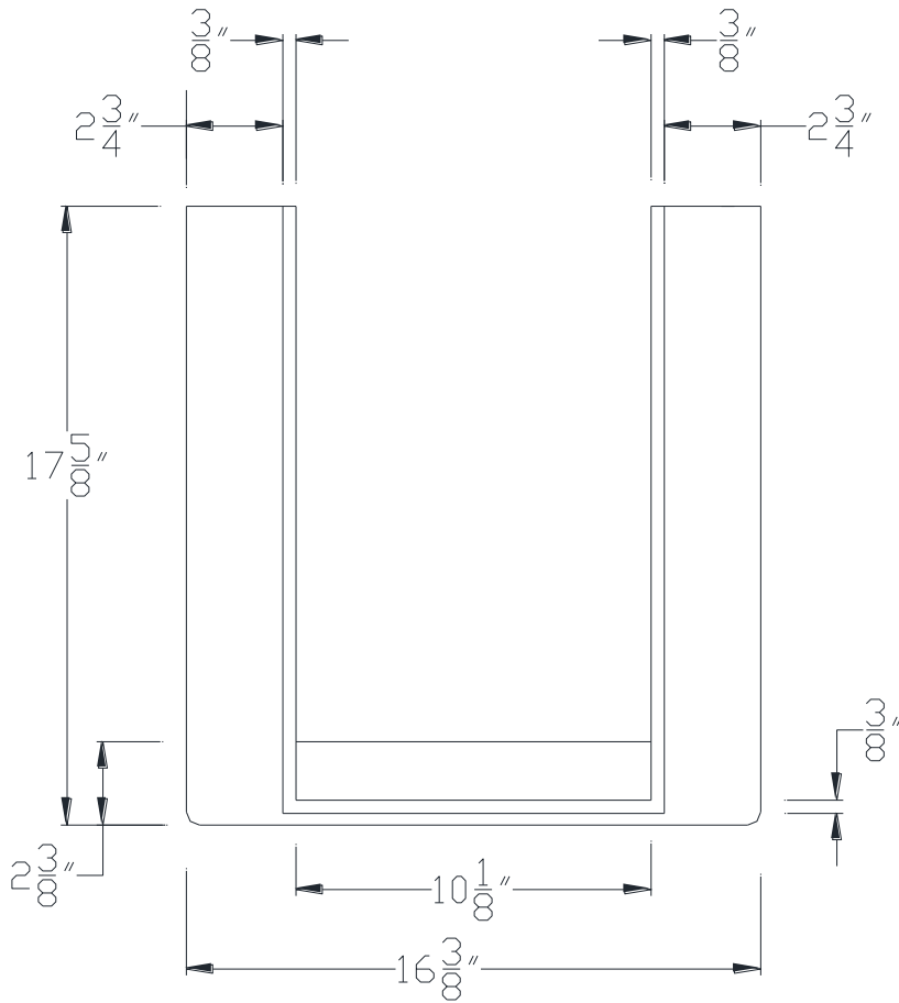
FRONT VIEW
