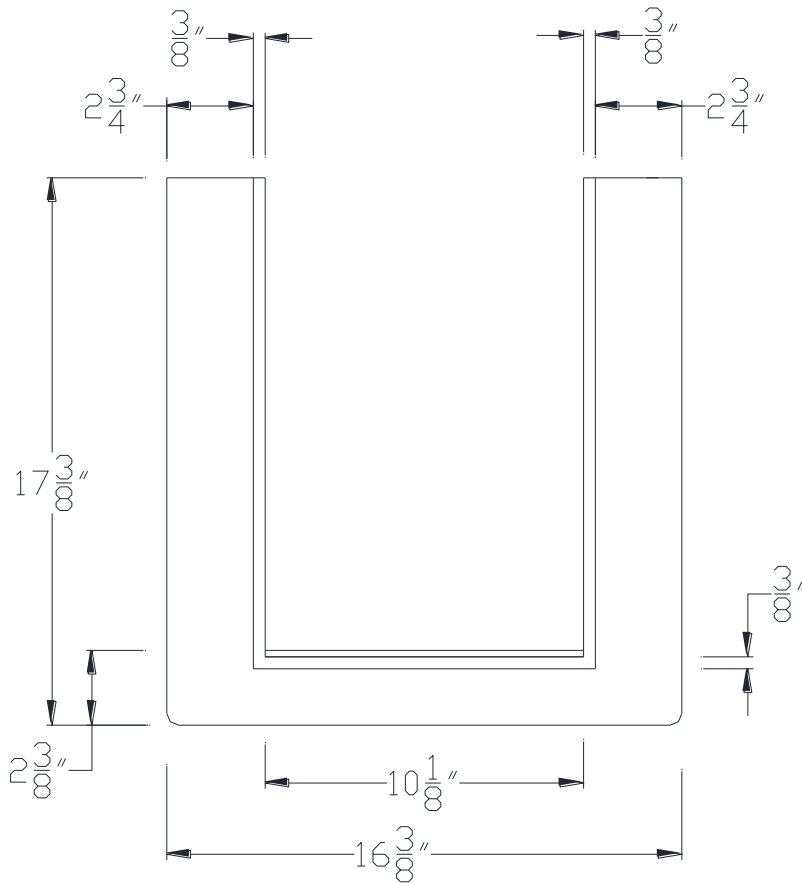
FRONT VIEW
