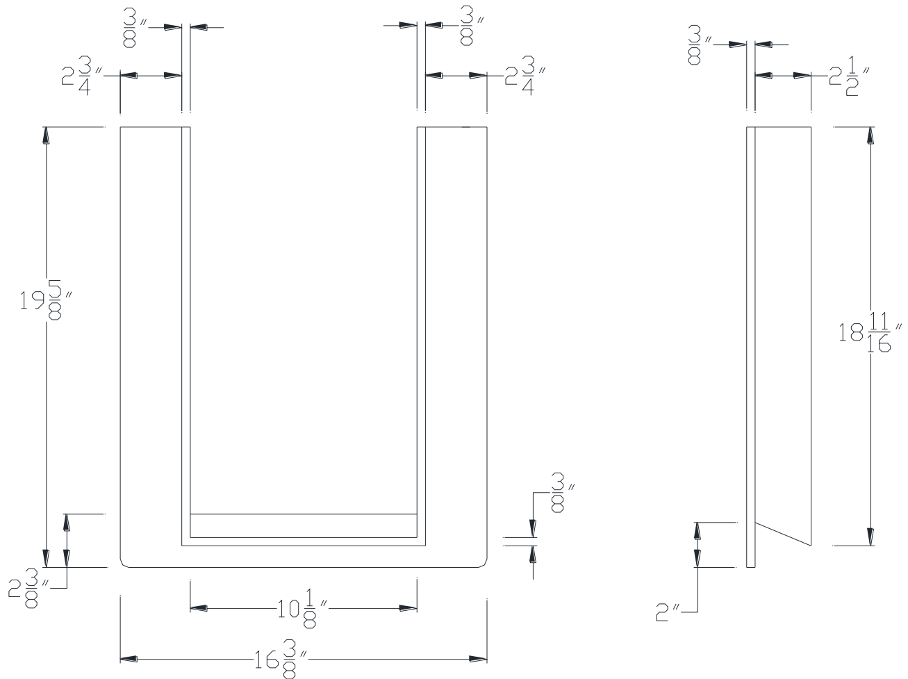
FRONT VIEW
