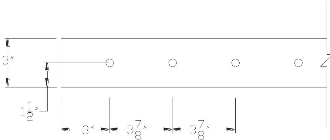
TOP VIEW
