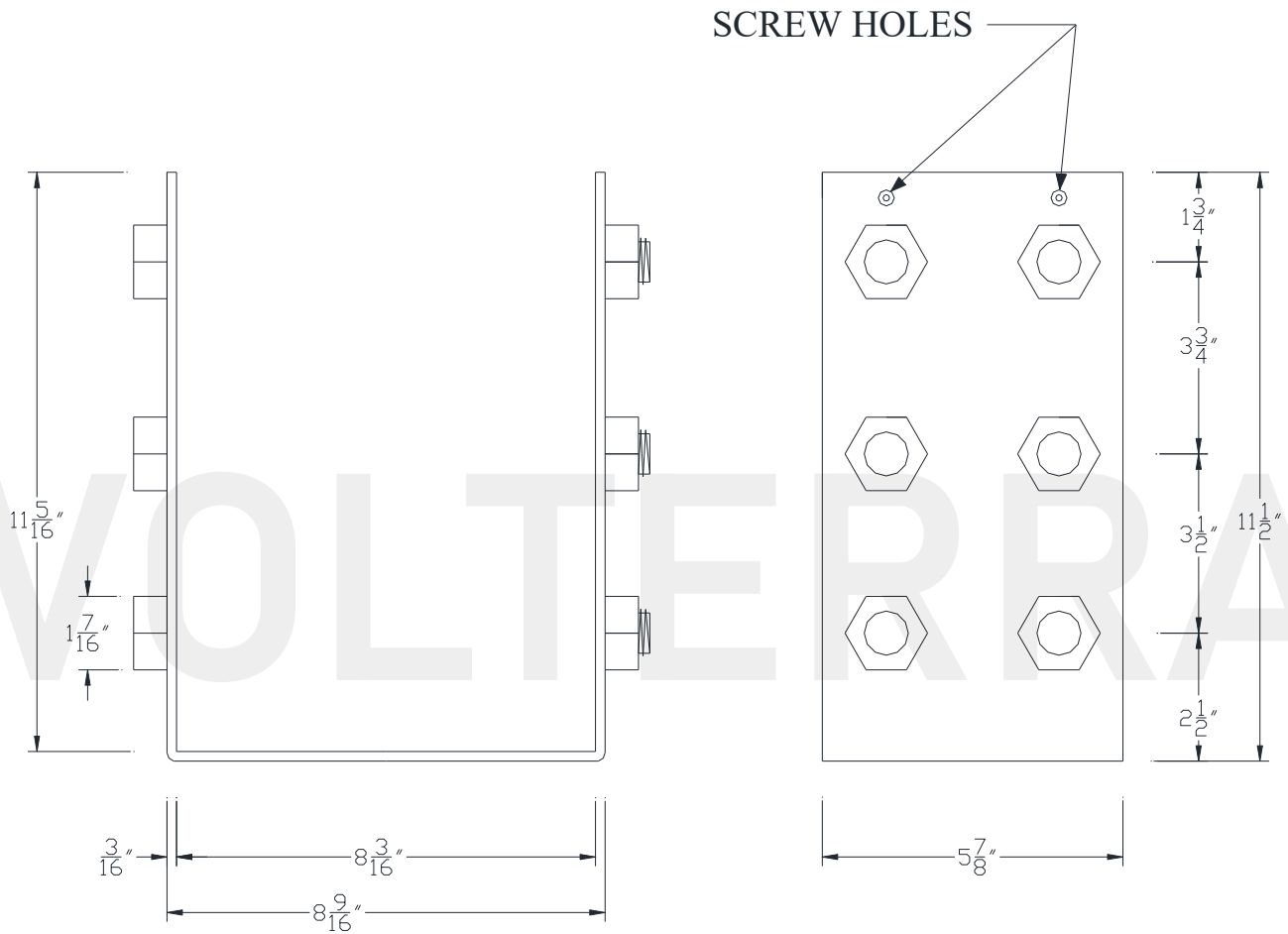
FRONT VIEW
