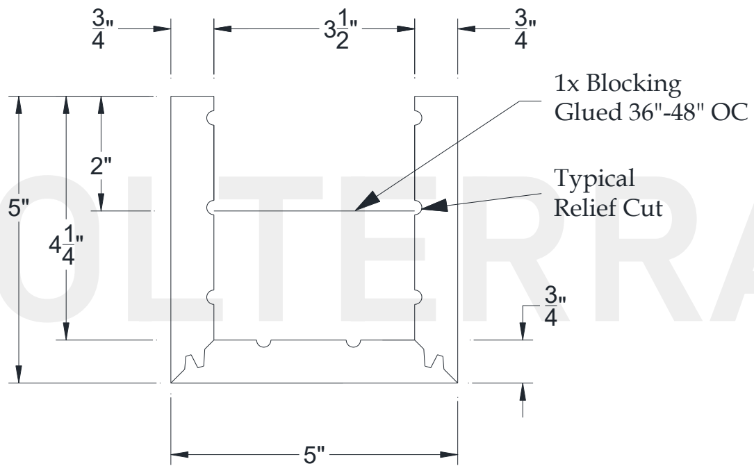
SECTIONAL VIEW
