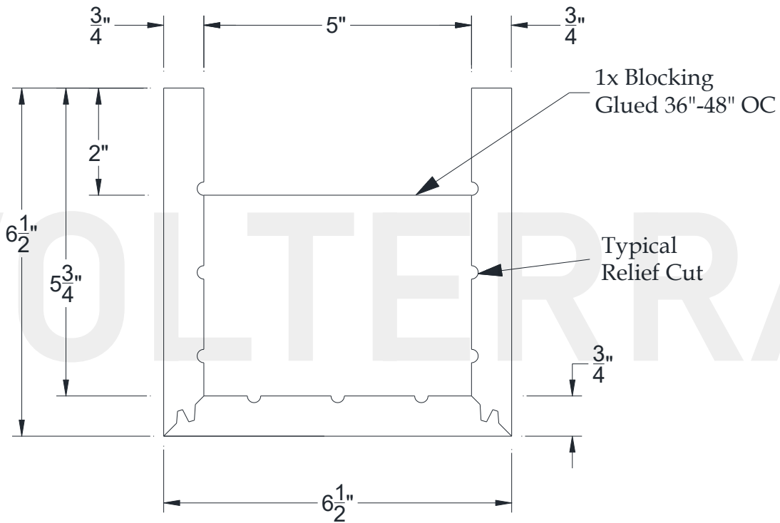
SECTIONAL VIEW
