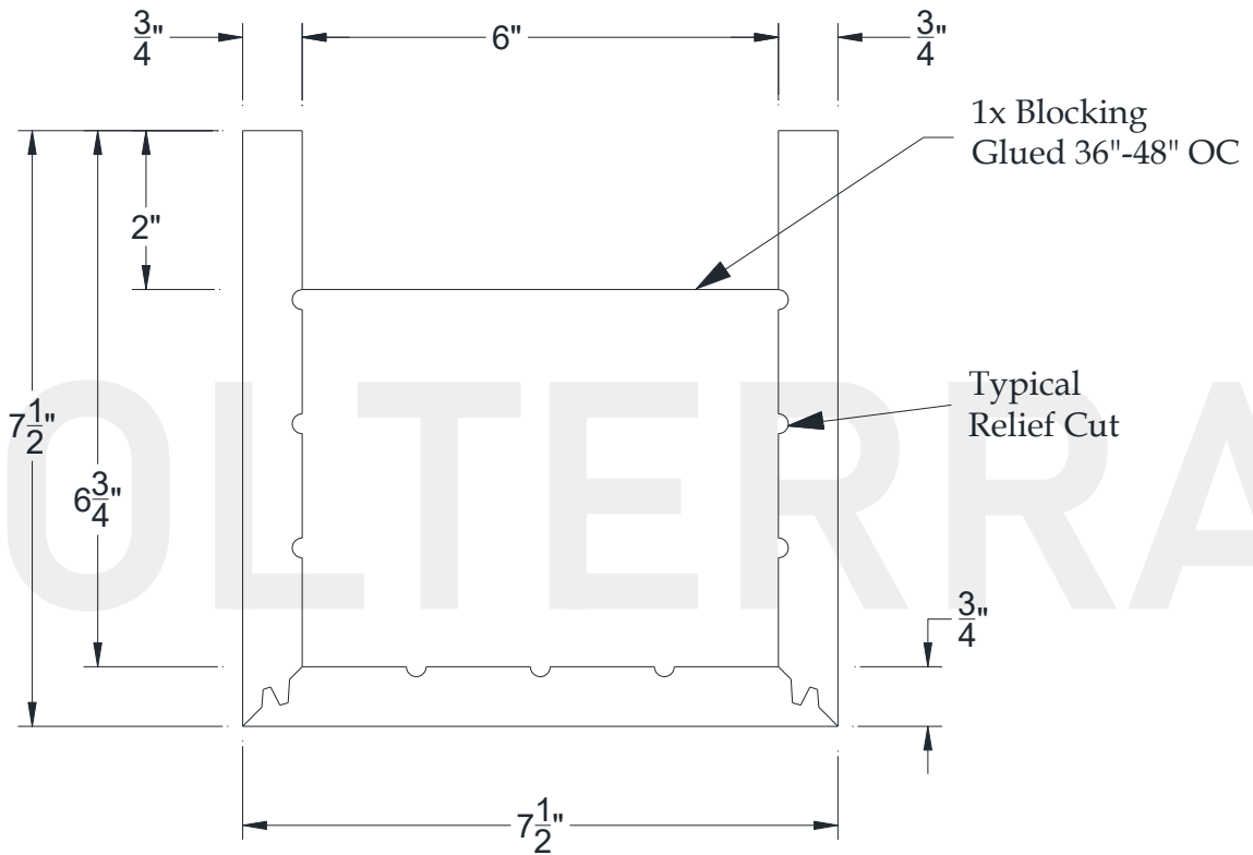
SECTIONAL VIEW
