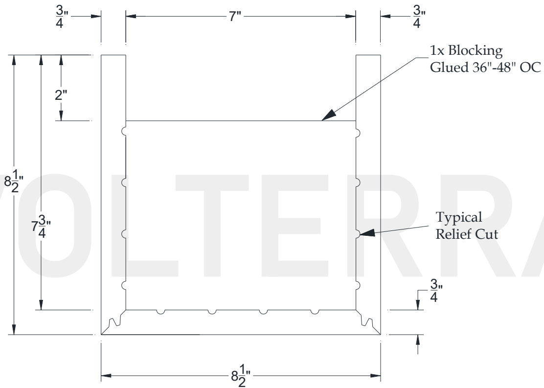
SECTIONAL VIEW
