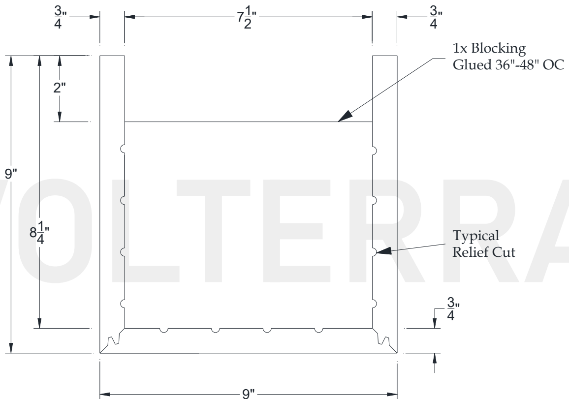
SECTIONAL VIEW
