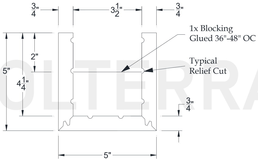
SECTIONAL VIEW
