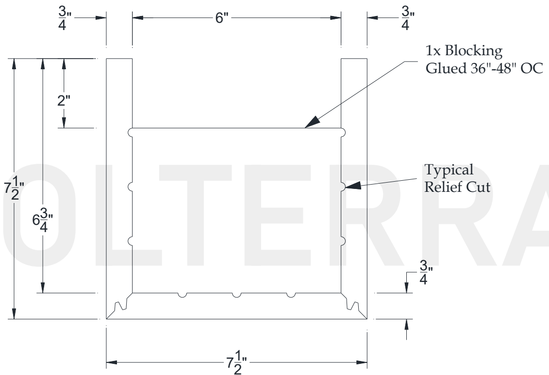
SECTIONAL VIEW
