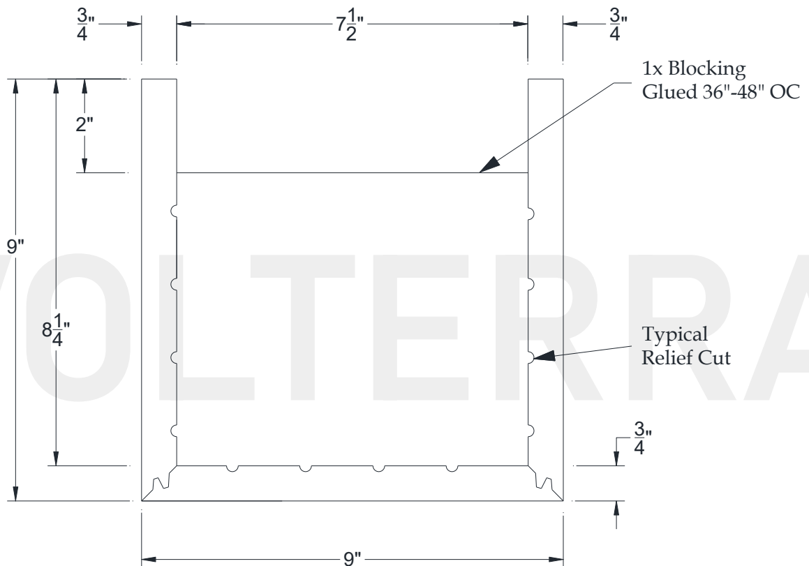
SECTIONAL VIEW
