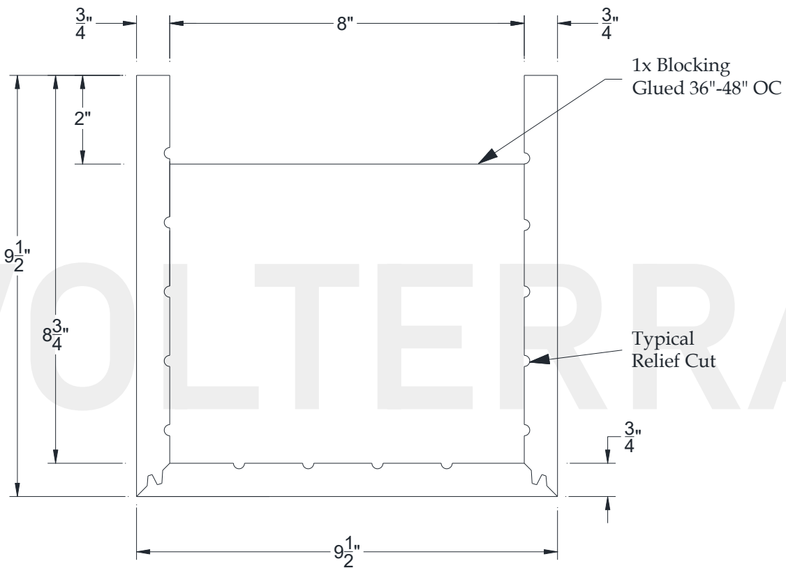
SECTIONAL VIEW
