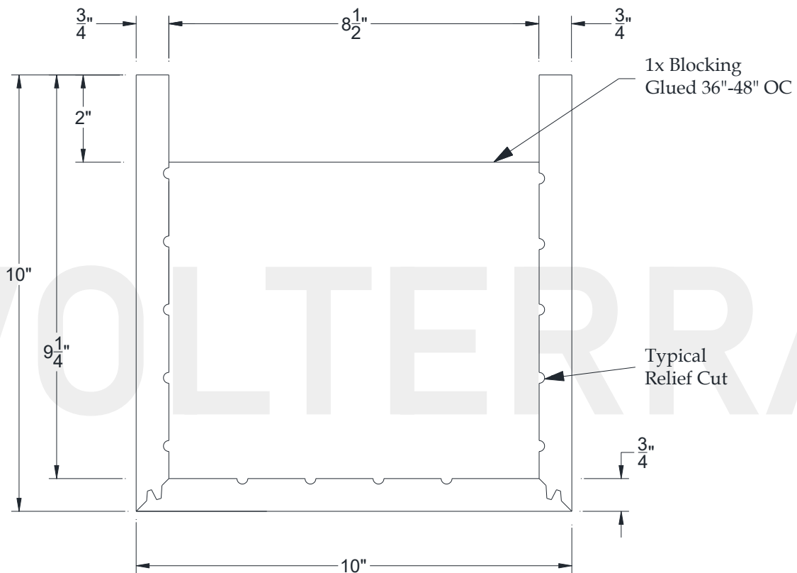
SECTIONAL VIEW
