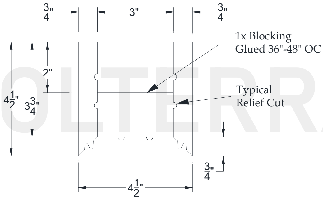
SECTIONAL VIEW
