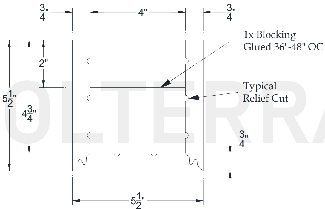
SECTIONAL VIEW
