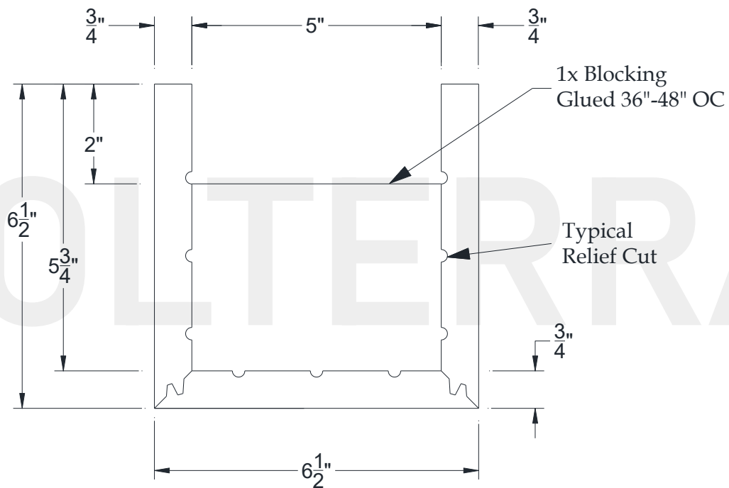
SECTIONAL VIEW
