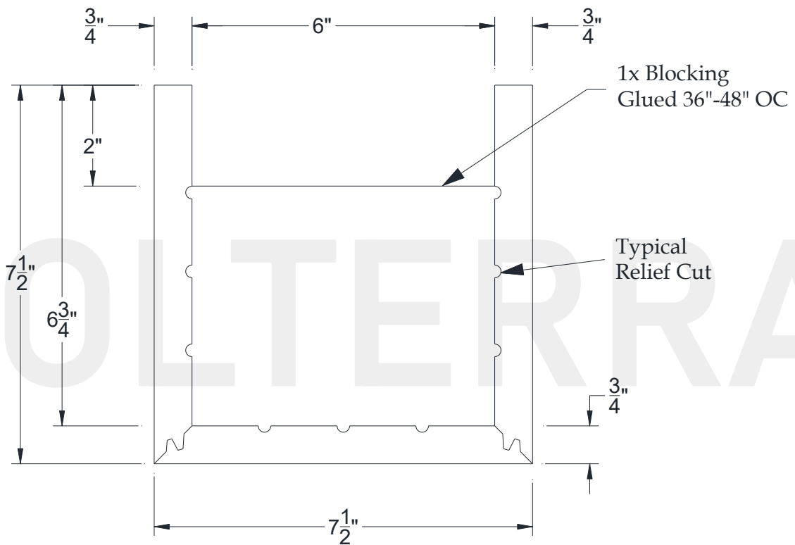
SECTIONAL VIEW
