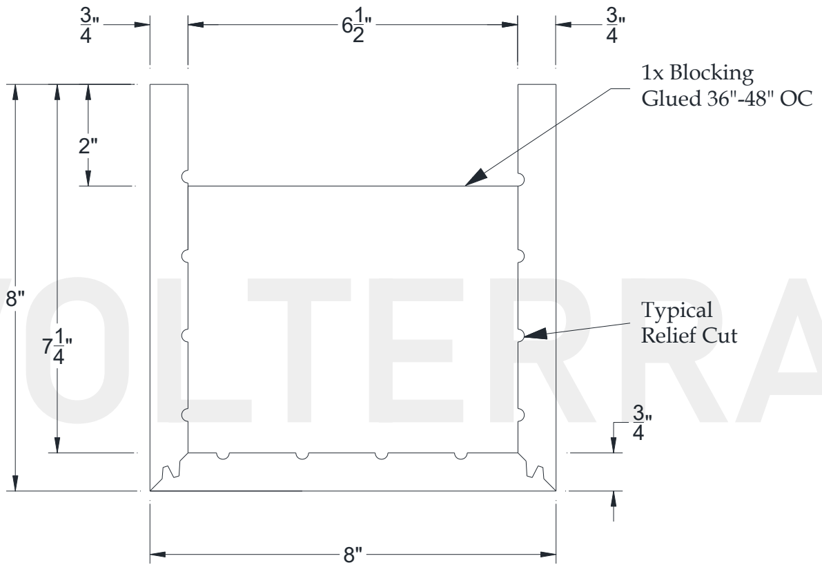
SECTIONAL VIEW
