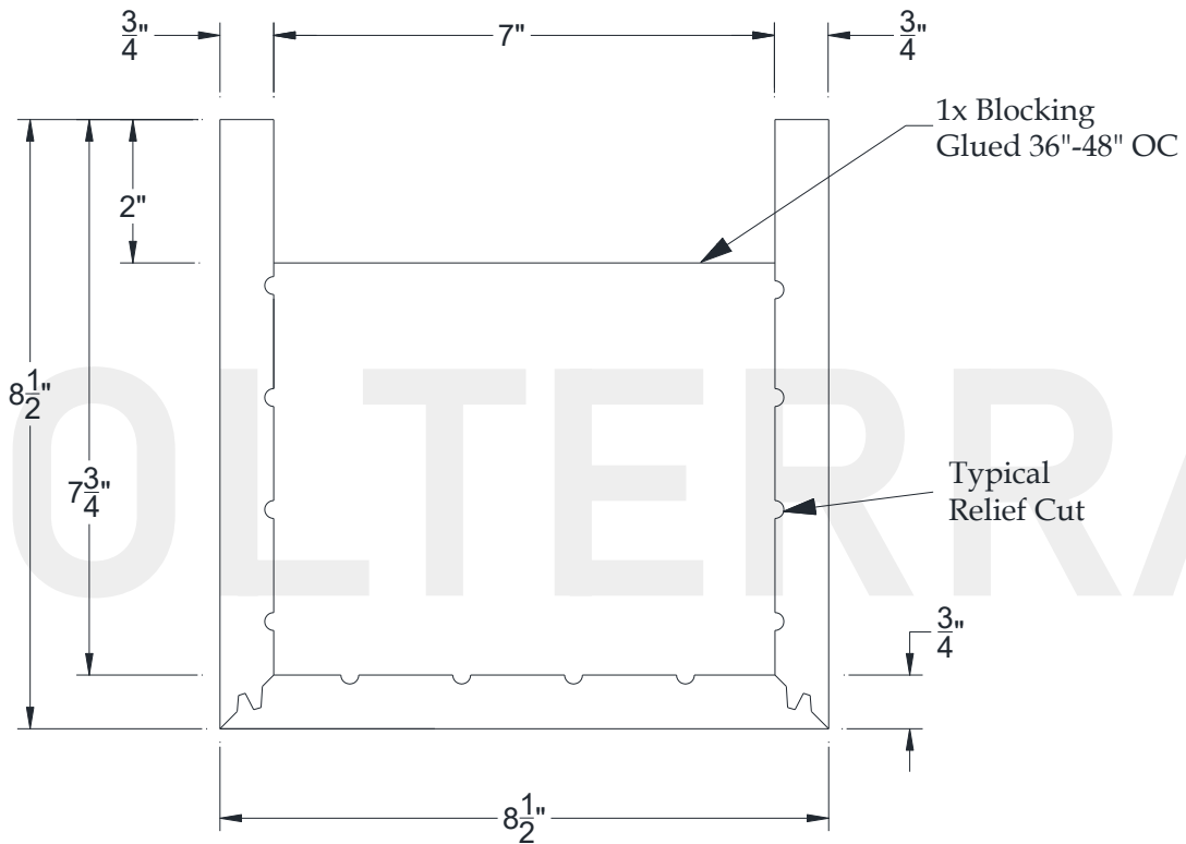
SECTIONAL VIEW
