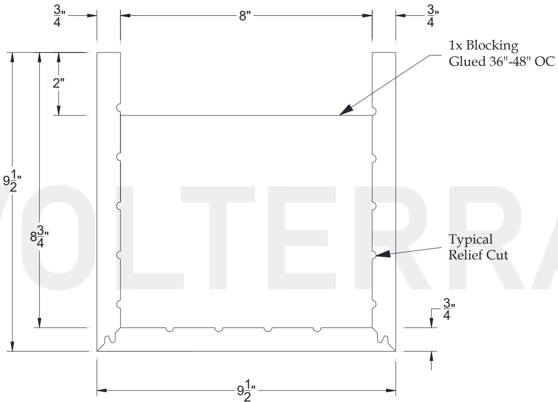
SECTIONAL VIEW
