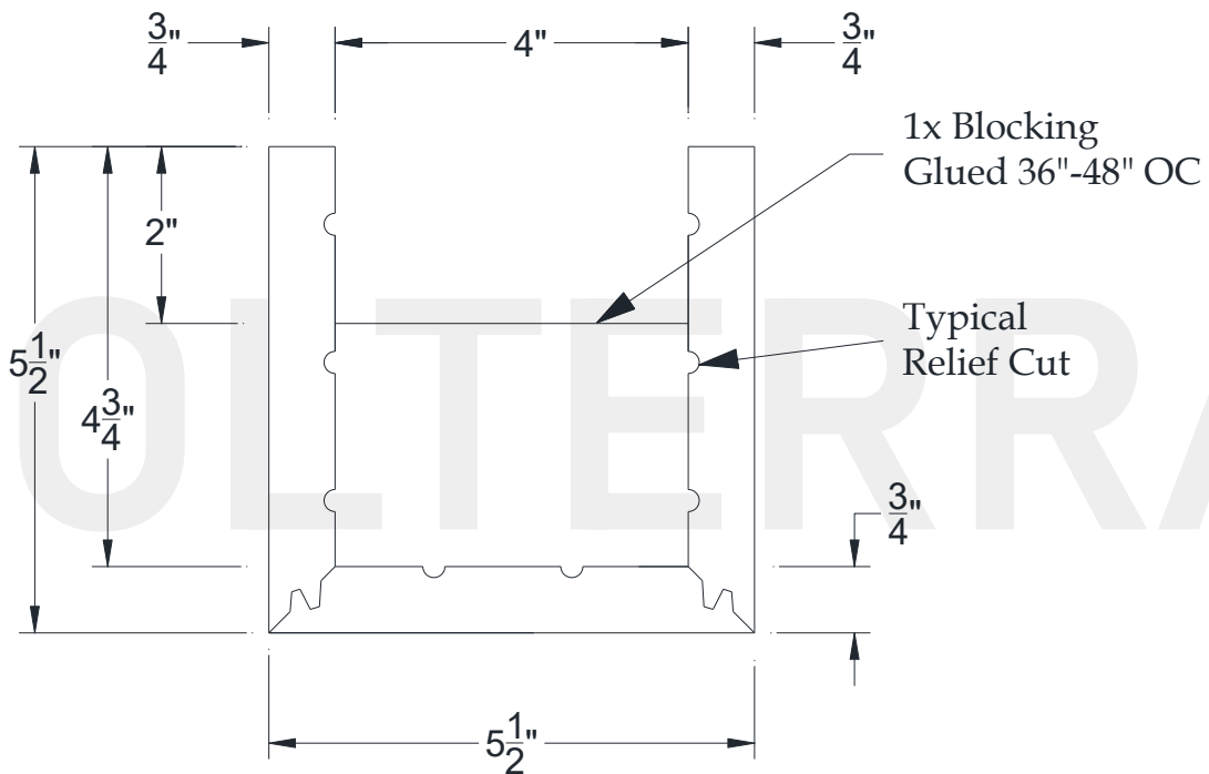
SECTIONAL VIEW
