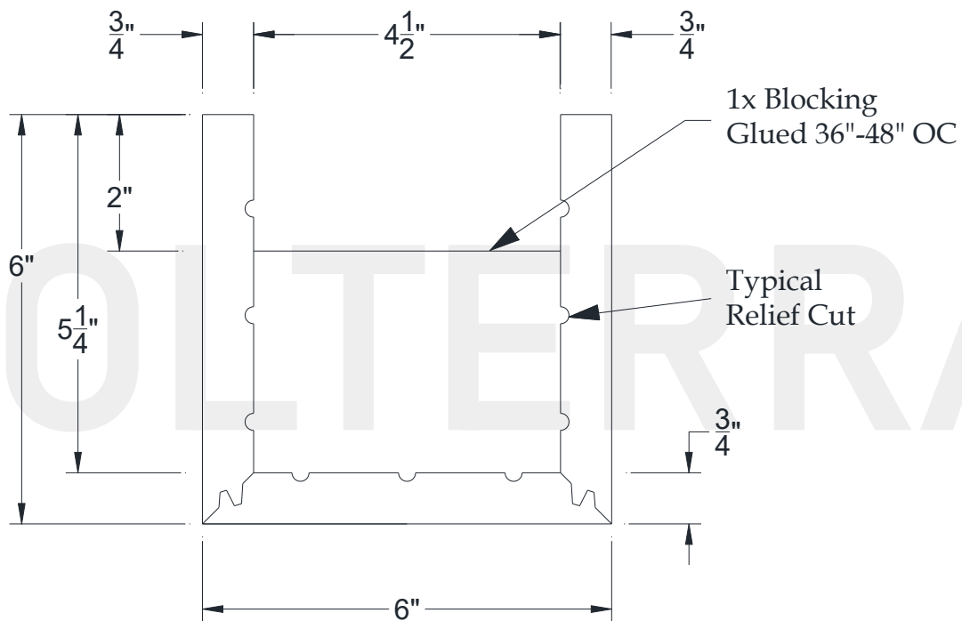
SECTIONAL VIEW
