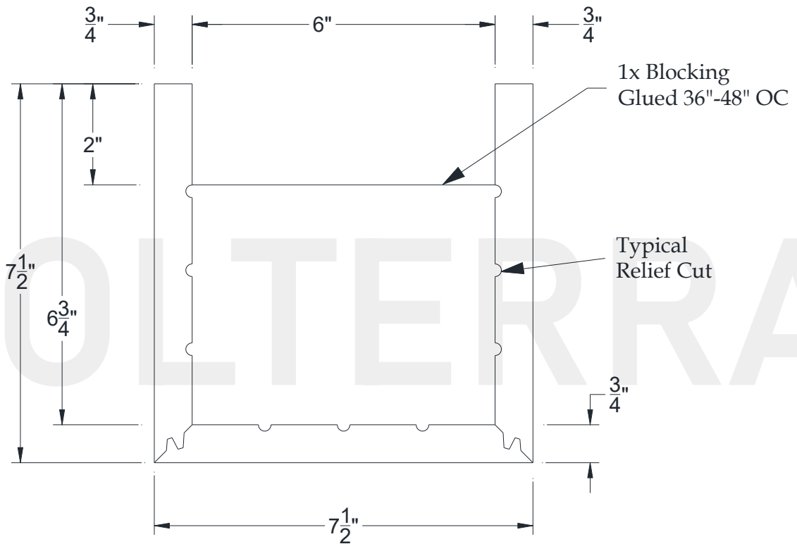
SECTIONAL VIEW
