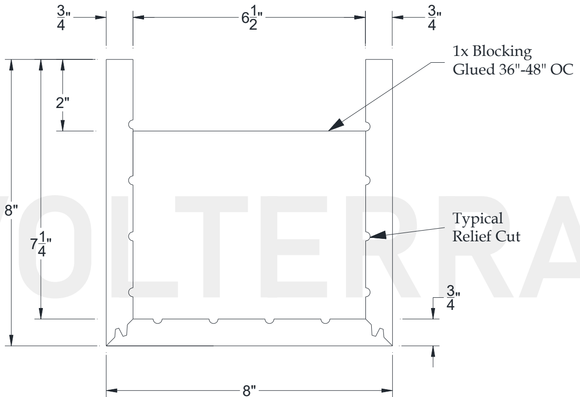
SECTIONAL VIEW
