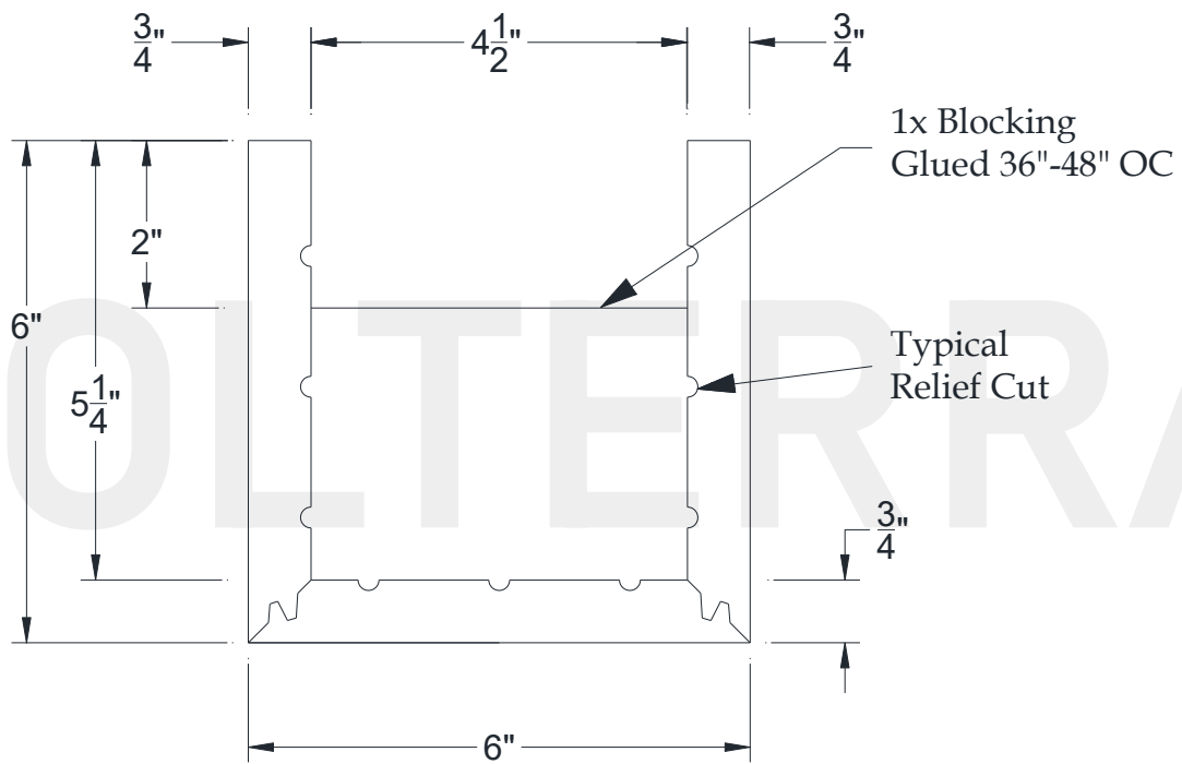
SECTIONAL VIEW
